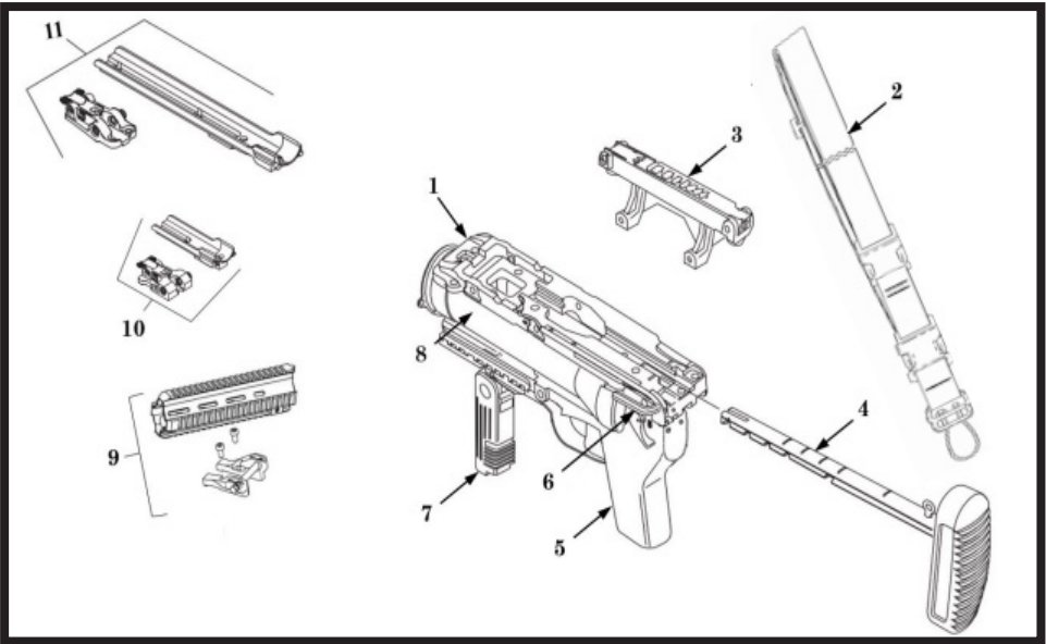
M320A1 Diagram
