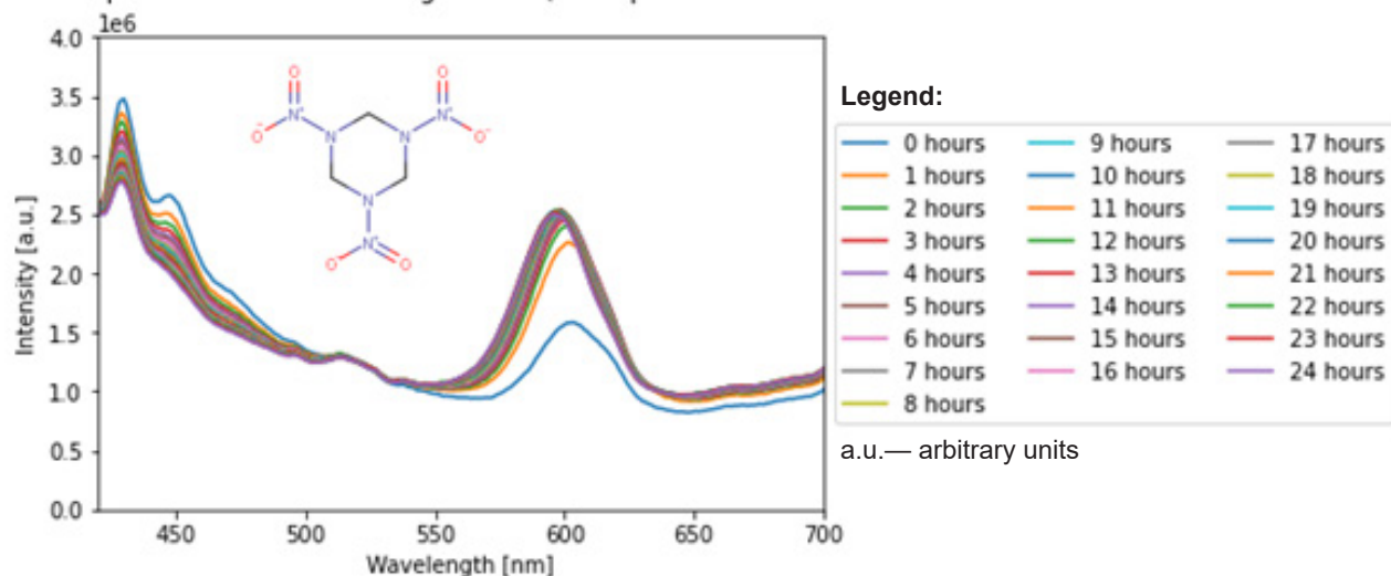
Figure 5. Measured quenching response of 2.0 mg of QD-doped PVC fiber to the presence of 0.5 mg of RDX
