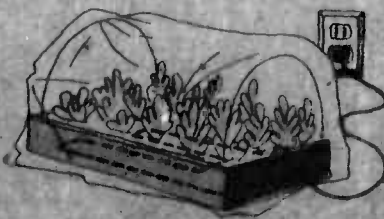
Succulent and herbaceous cuttings root readily if given bottom heat and constant humidity. An electric heating cable with a plastic cover positioned in the bottom of a flat is ideal.
